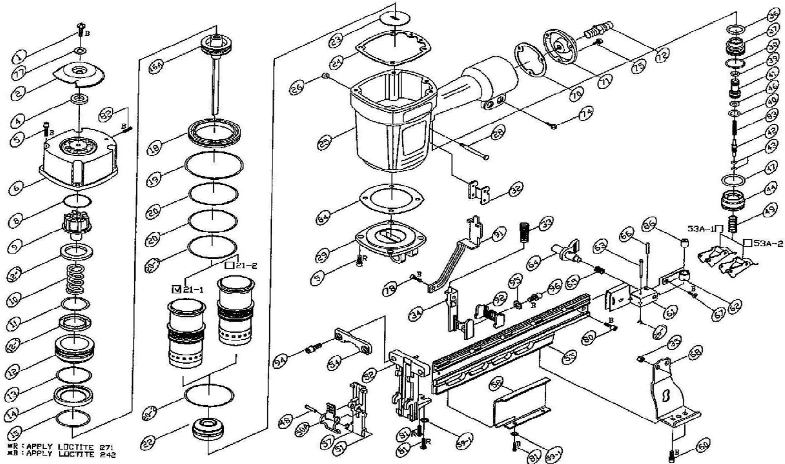
VA0359 HEAVY DUTY STAPLER
